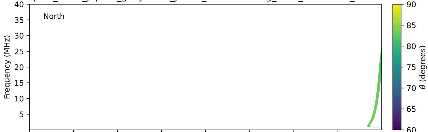
expres_earth_jupiter_ganymede_jrm33_lossc-wid1deg_3kev_20161011_v11.cdf
