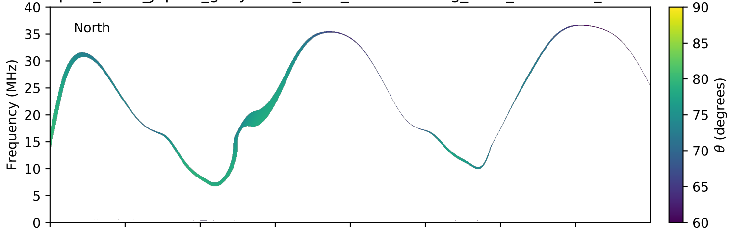
expres_earth_jupiter_ganymede_isaac_lossc-wid1deg_5kev_20161031_v01.cdf
