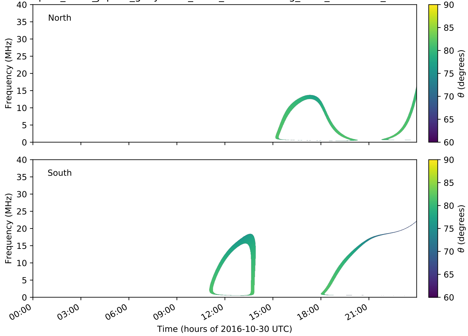
expres_earth_jupiter_ganymede_isaac_lossc-wid1deg_5kev_20161030_v01.cdf
