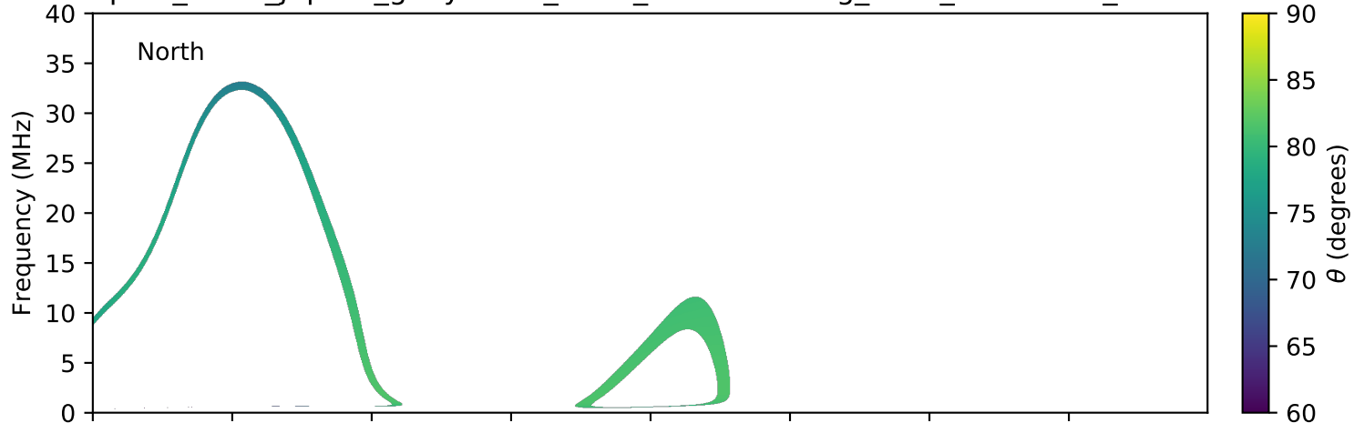
expres_earth_jupiter_ganymede_isaac_lossc-wid1deg_5kev_20161019_v01.cdf
