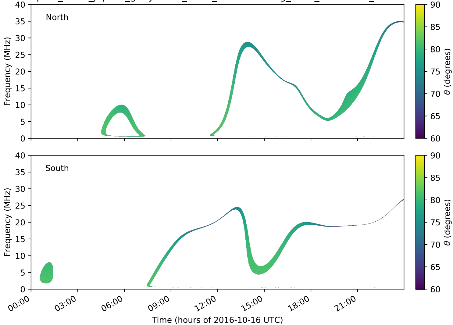
expres_earth_jupiter_ganymede_isaac_lossc-wid1deg_5kev_20161016_v01.cdf
