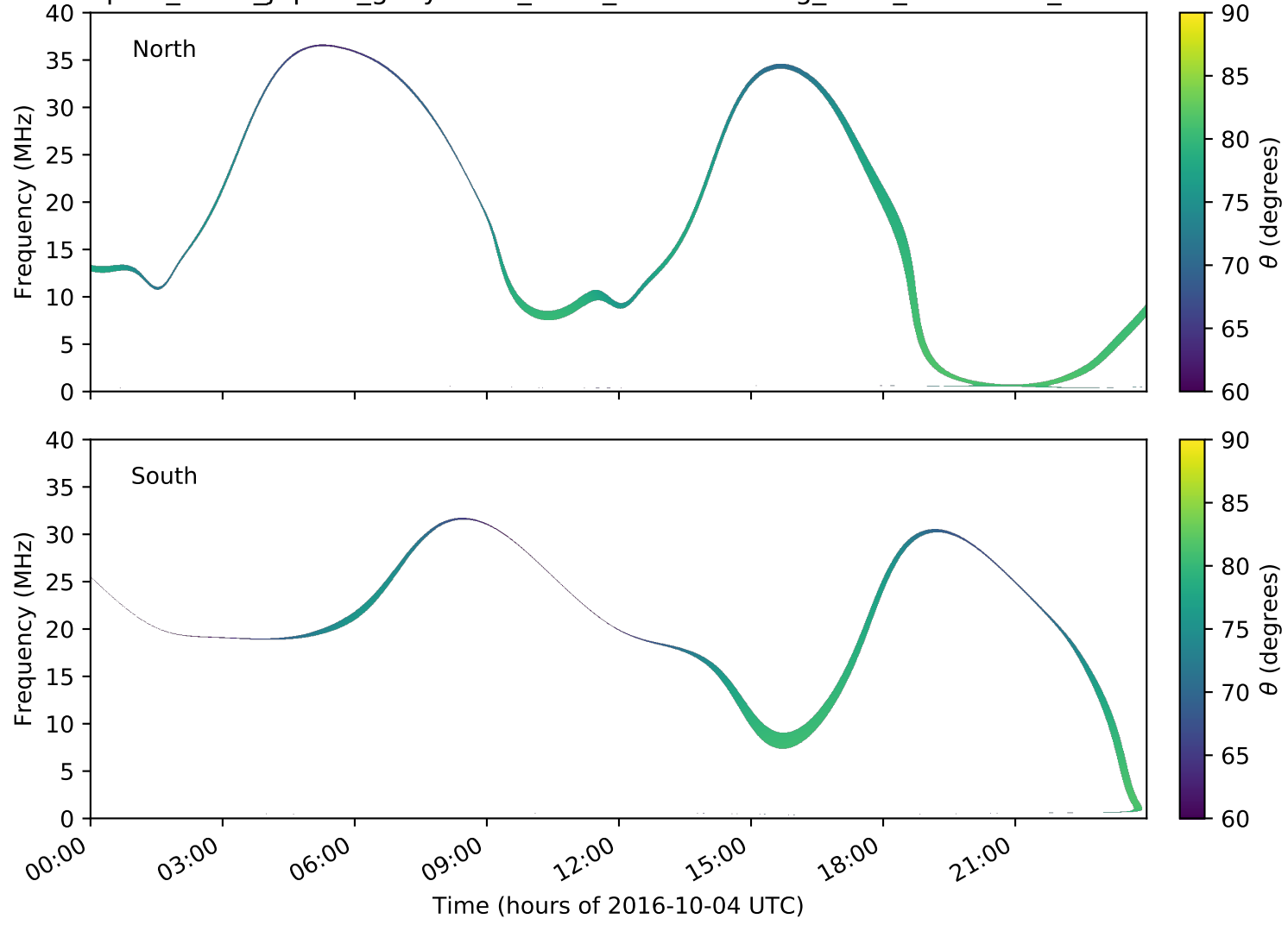
expres_earth_jupiter_ganymede_isaac_lossc-wid1deg_5kev_20161004_v01.cdf
