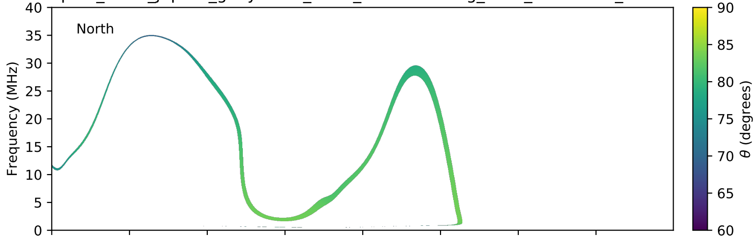
expres_earth_jupiter_ganymede_isaac_lossc-wid1deg_3kev_20161026_v01.cdf
