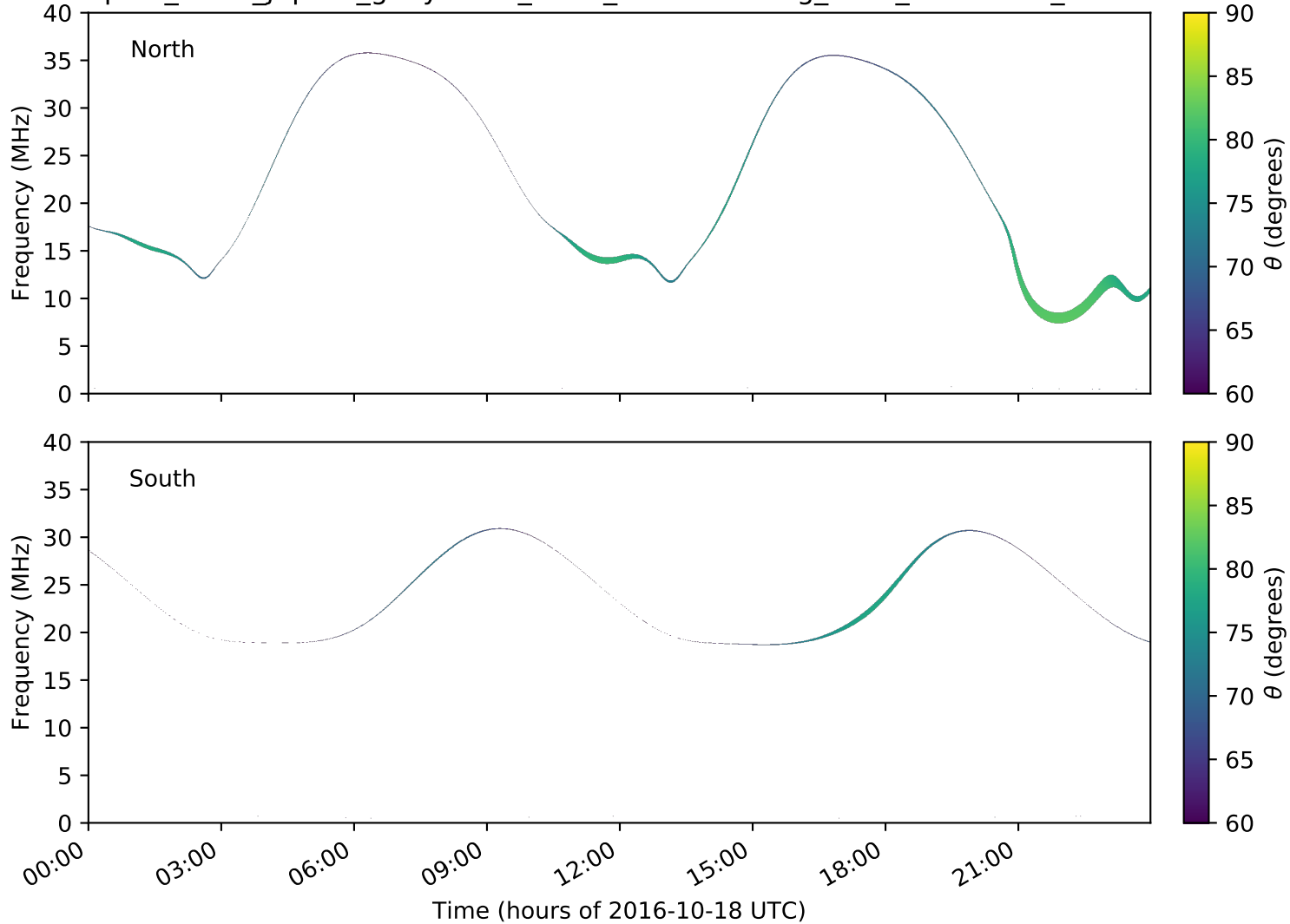
expres_earth_jupiter_ganymede_isaac_lossc-wid1deg_3kev_20161018_v01.cdf
