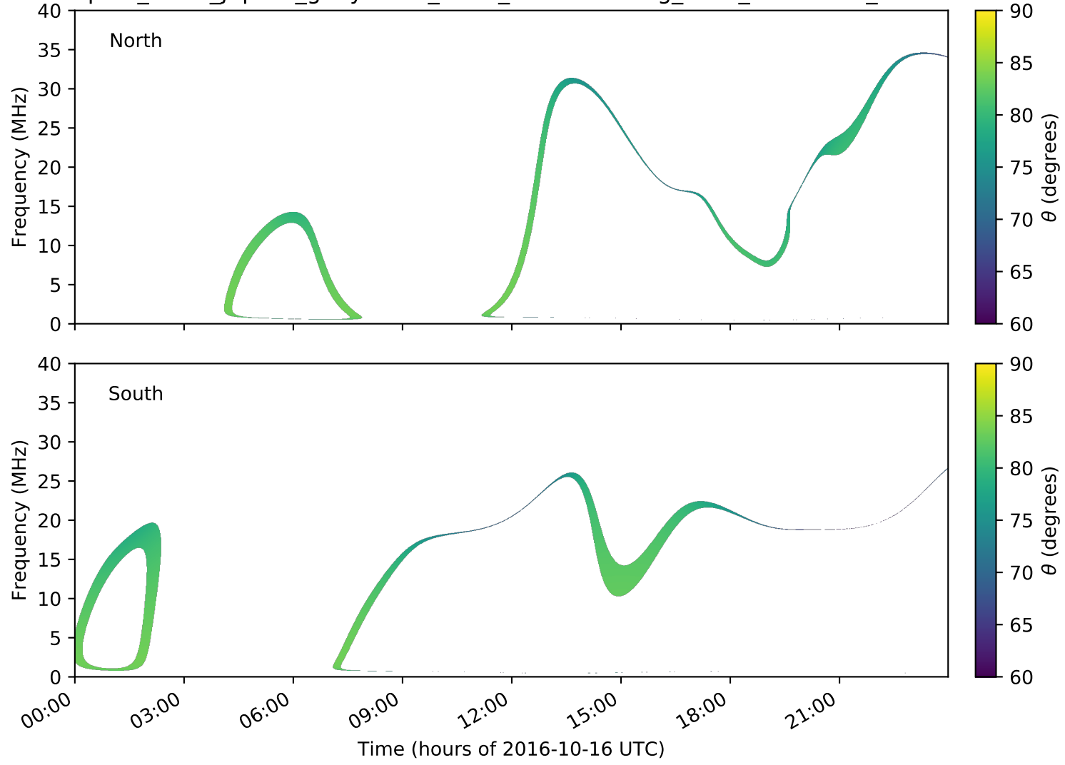
expres_earth_jupiter_ganymede_isaac_lossc-wid1deg_3kev_20161016_v01.cdf
