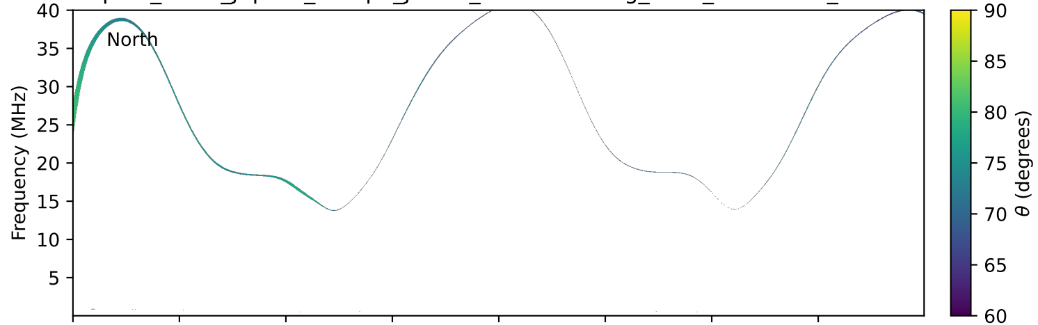
expres_earth_jupiter_europa_jrm33_lossc-wid1deg_3kev_20161019_v11.cdf
