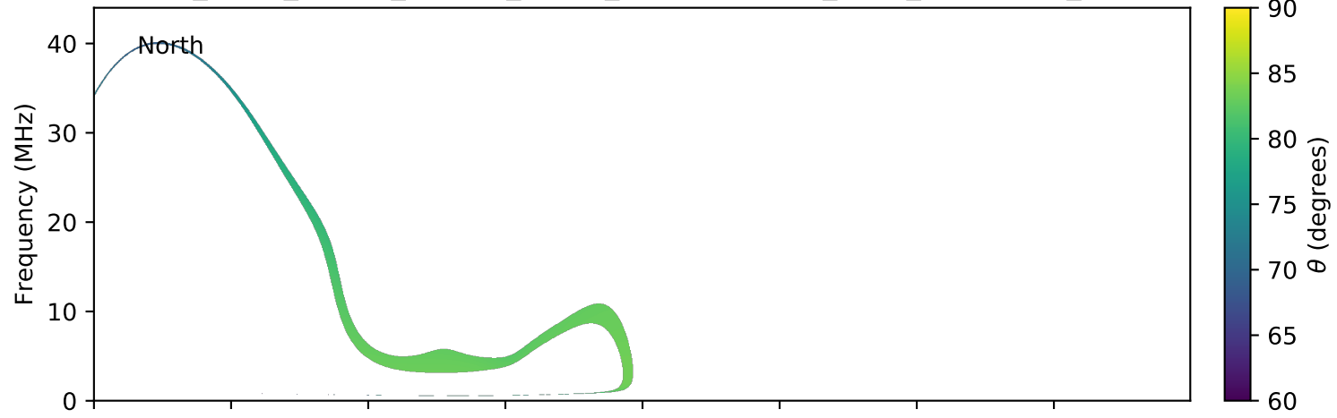
expres_earth_jupiter_europa_jrm09_lossc-wid1deg_3kev_20161029_v01.cdf
