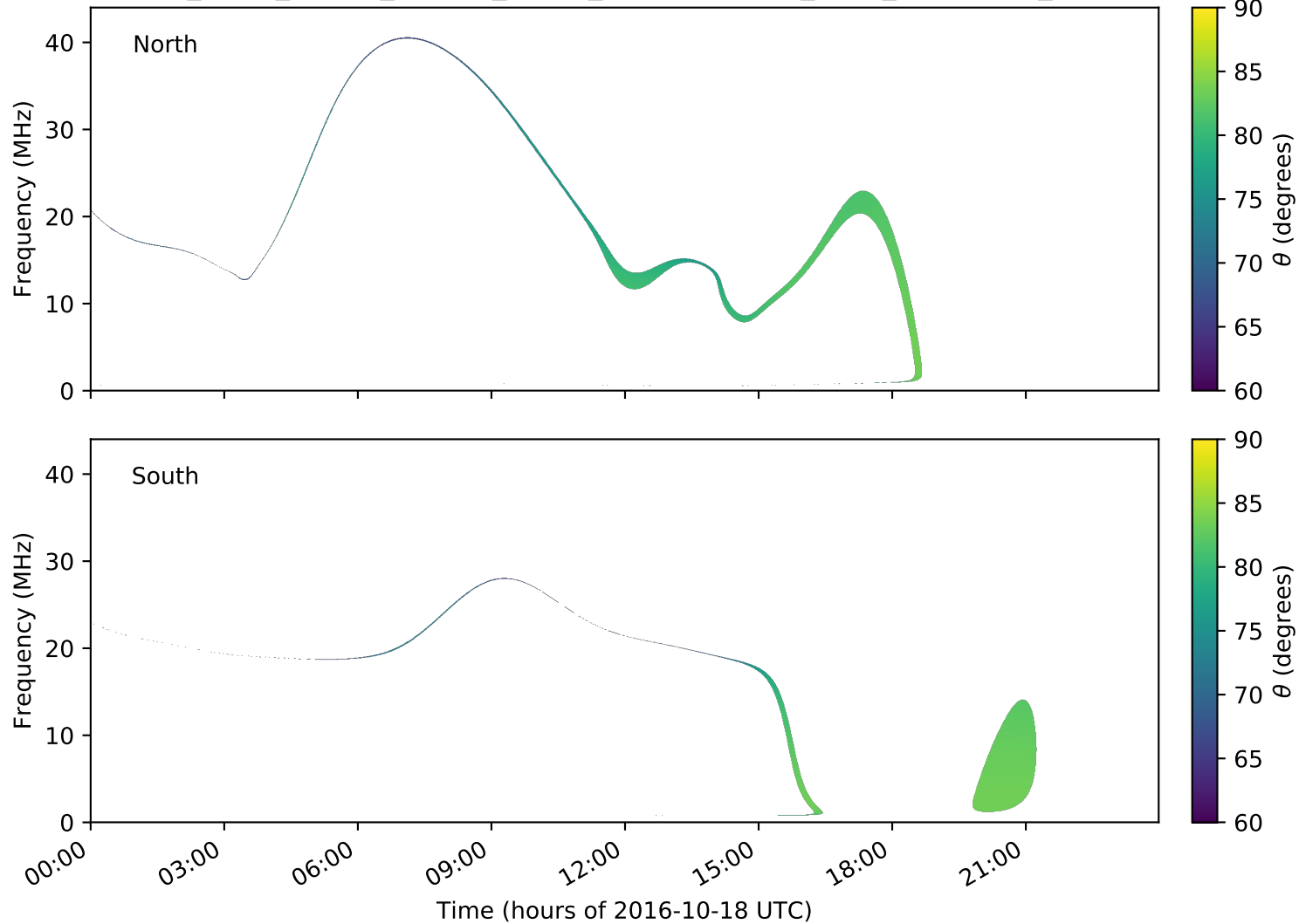
expres_earth_jupiter_europa_jrm09_lossc-wid1deg_3kev_20161018_v01.cdf
