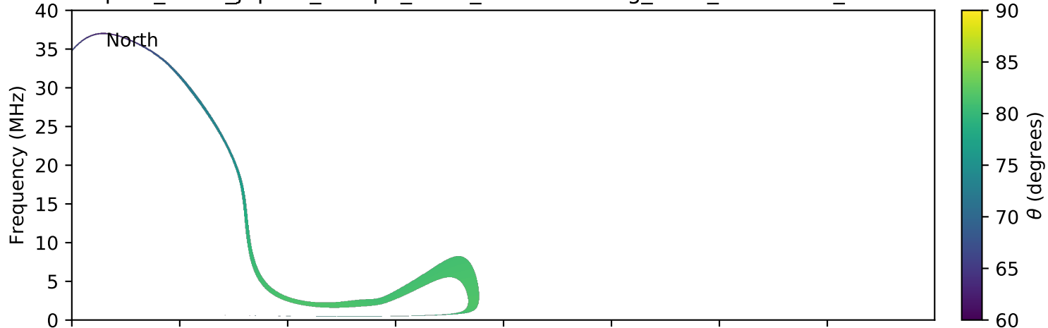
expres_earth_jupiter_europa_isaac_lossc-wid1deg_5kev_20161029_v01.cdf
