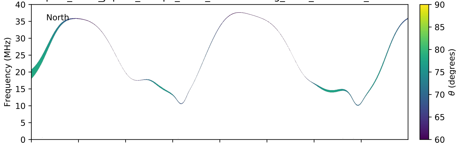
expres_earth_jupiter_europa_isaac_lossc-wid1deg_5kev_20161021_v01.cdf
