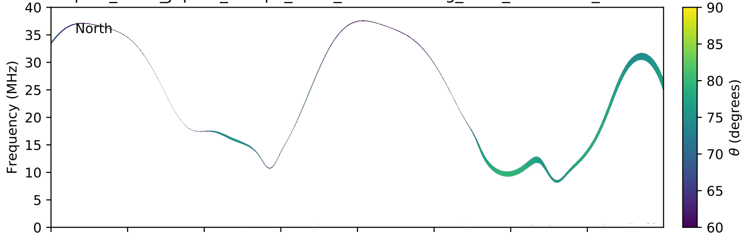
expres_earth_jupiter_europa_isaac_lossc-wid1deg_5kev_20161007_v01.cdf
