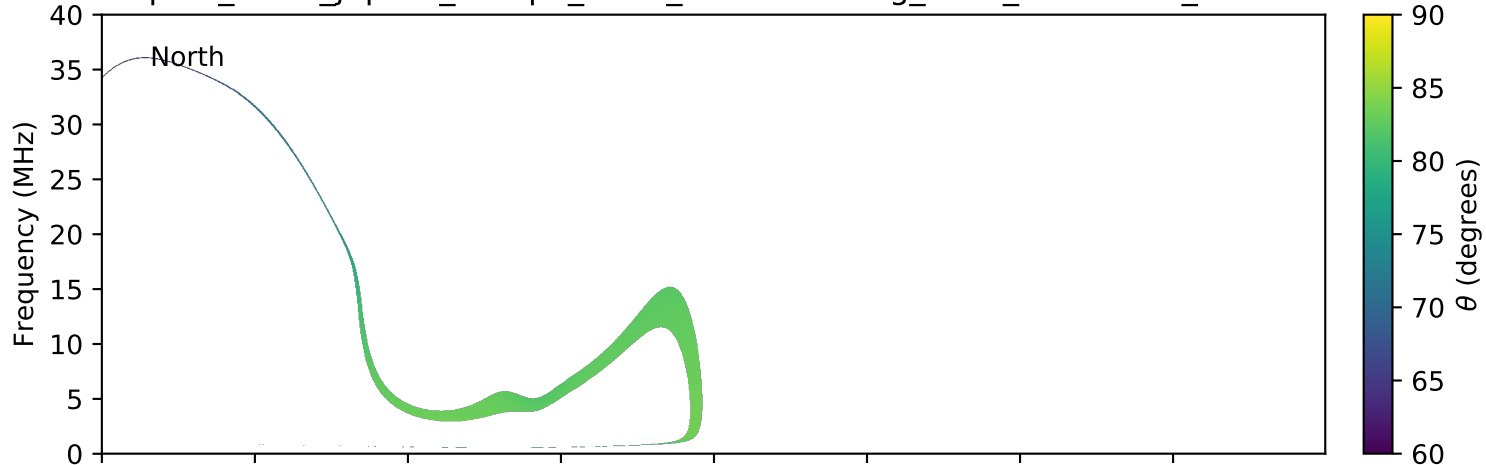
expres_earth_jupiter_europa_isaac_lossc-wid1deg_3kev_20161029_v01.cdf
