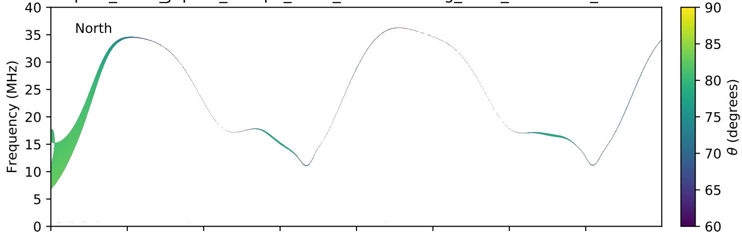
expres_earth_jupiter_europa_isaac_lossc-wid1deg_3kev_20161028_v01.cdf
