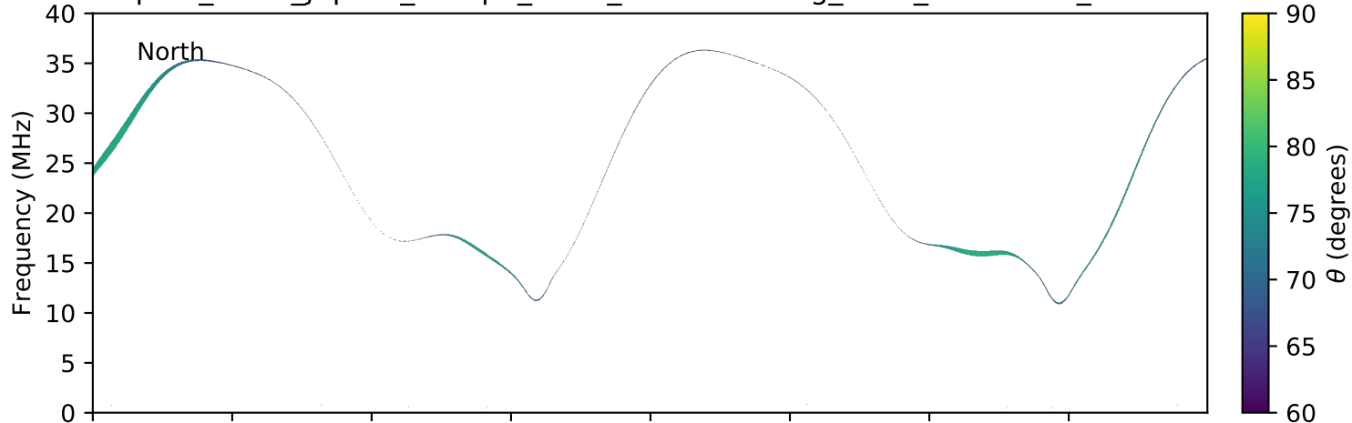
expres_earth_jupiter_europa_isaac_lossc-wid1deg_3kev_20161021_v01.cdf
