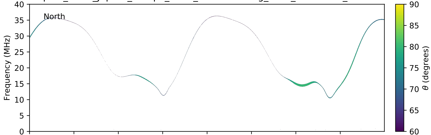
expres_earth_jupiter_europa_isaac_lossc-wid1deg_3kev_20161014_v01.cdf
