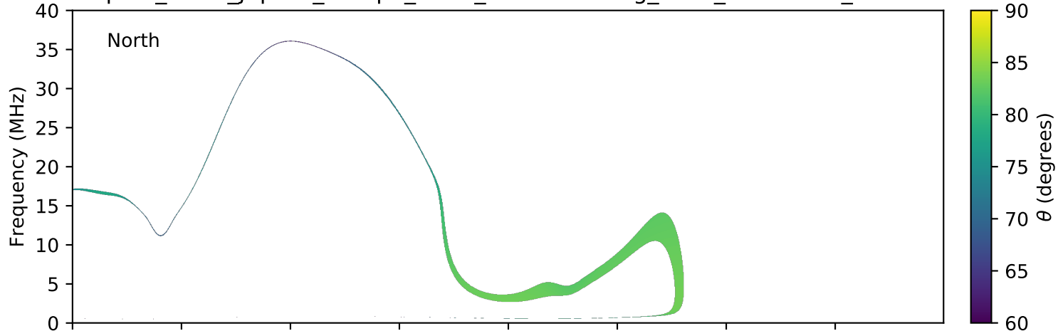
expres_earth_jupiter_europa_isaac_lossc-wid1deg_3kev_20161011_v01.cdf
