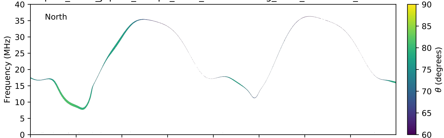
expres_earth_jupiter_europa_isaac_lossc-wid1deg_3kev_20161003_v01.cdf
