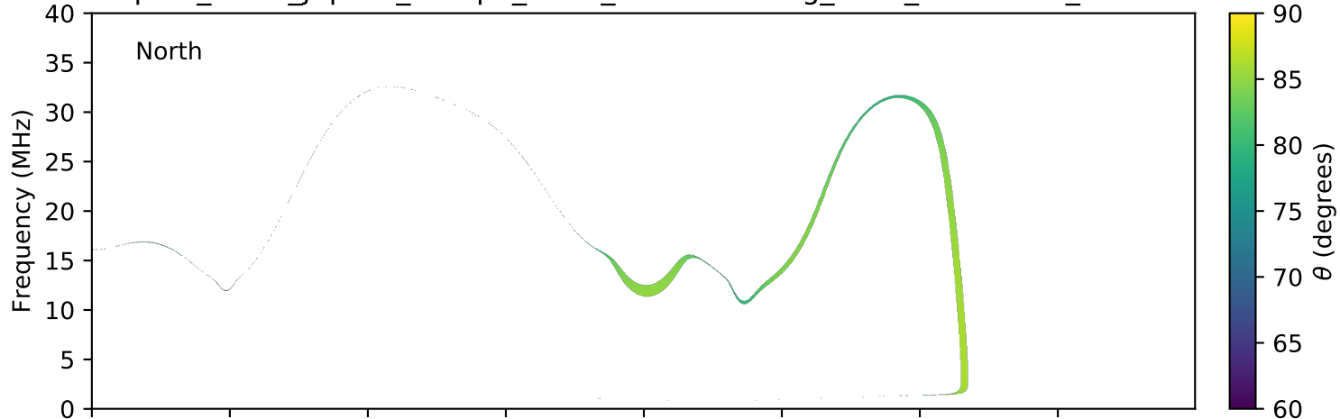
expres_earth_jupiter_europa_isaac_lossc-wid1deg_1kev_20161018_v01.cdf
