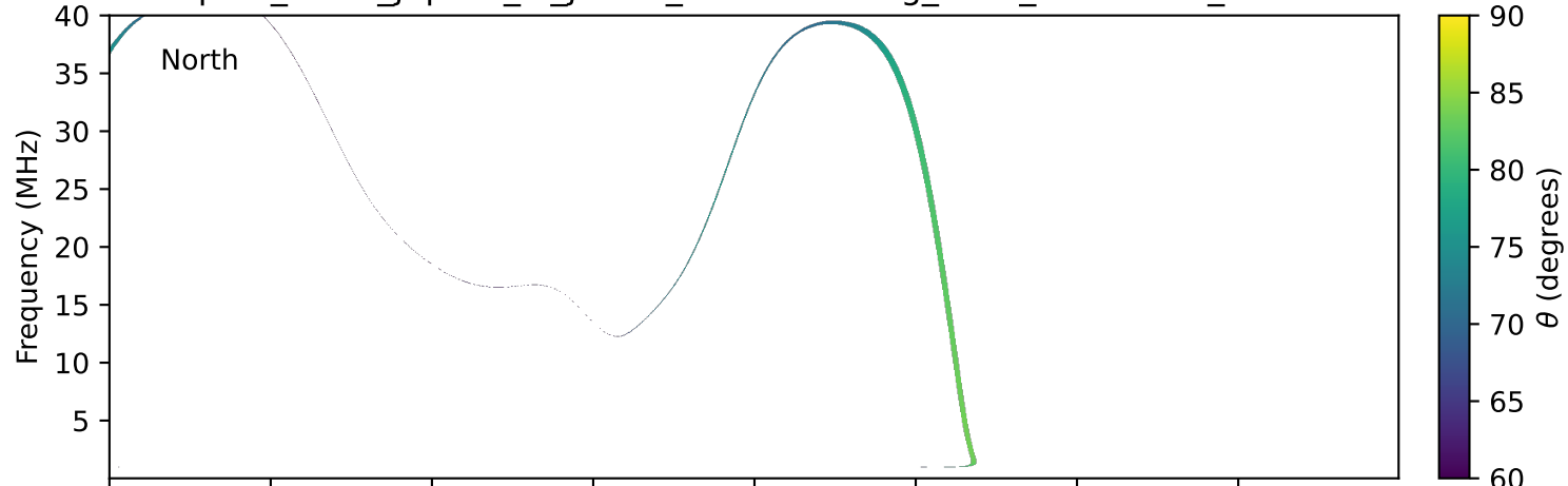
expres_earth_jupiter_io_jrm33_lossc-wid1deg_3kev_20160925_v11.cdf
