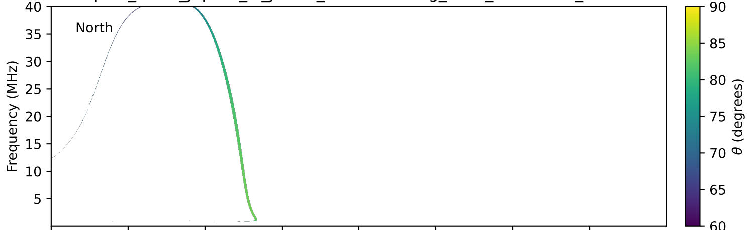
expres_earth_jupiter_io_jrm33_lossc-wid1deg_3kev_20160920_v11.cdf
