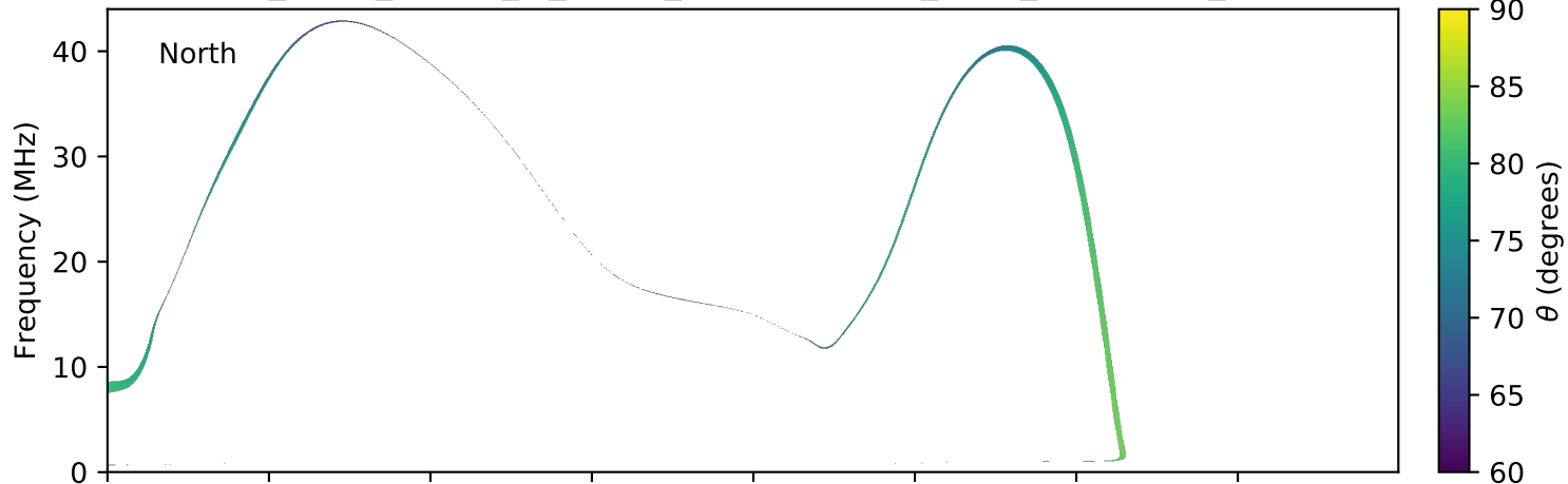
expres_earth_jupiter_io_jrm09_lossc-wid1deg_3kev_20160929_v01.cdf
