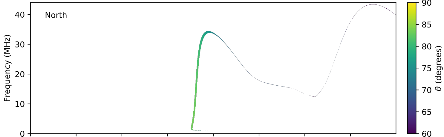
expres_earth_jupiter_io_jrm09_lossc-wid1deg_3kev_20160925_v01.cdf
