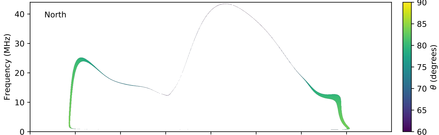
expres_earth_jupiter_io_jrm09_lossc-wid1deg_3kev_20160920_v01.cdf
