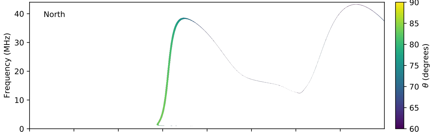
expres_earth_jupiter_io_jrm09_lossc-wid1deg_3kev_20160918_v01.cdf
