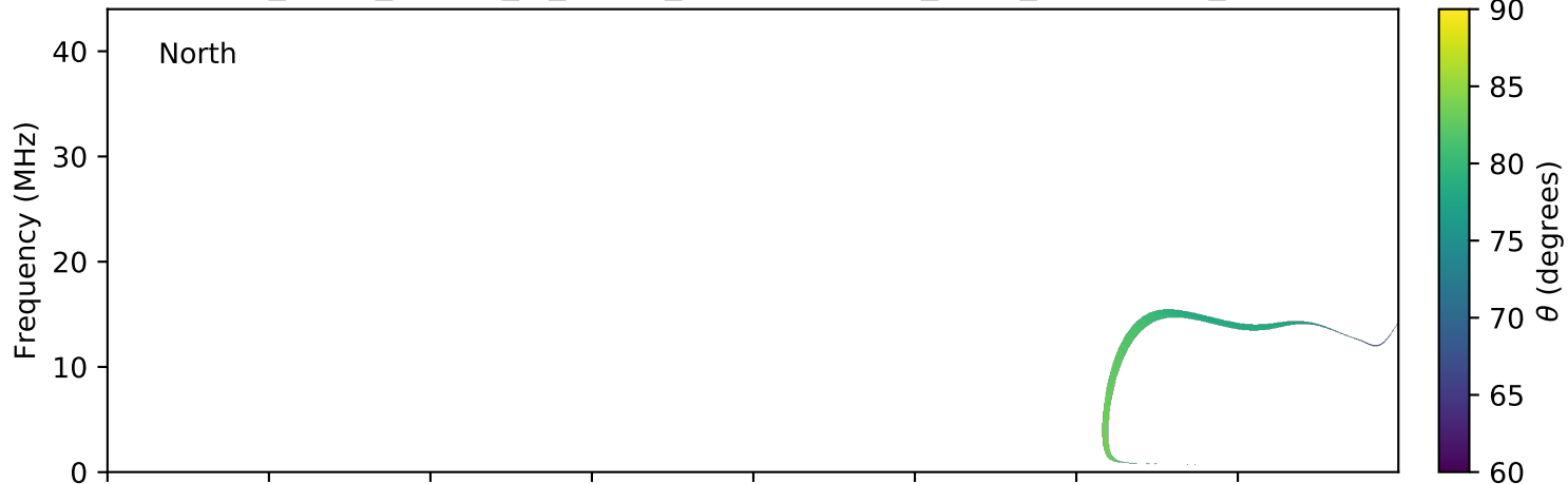
expres_earth_jupiter_io_jrm09_lossc-wid1deg_3kev_20160914_v01.cdf
