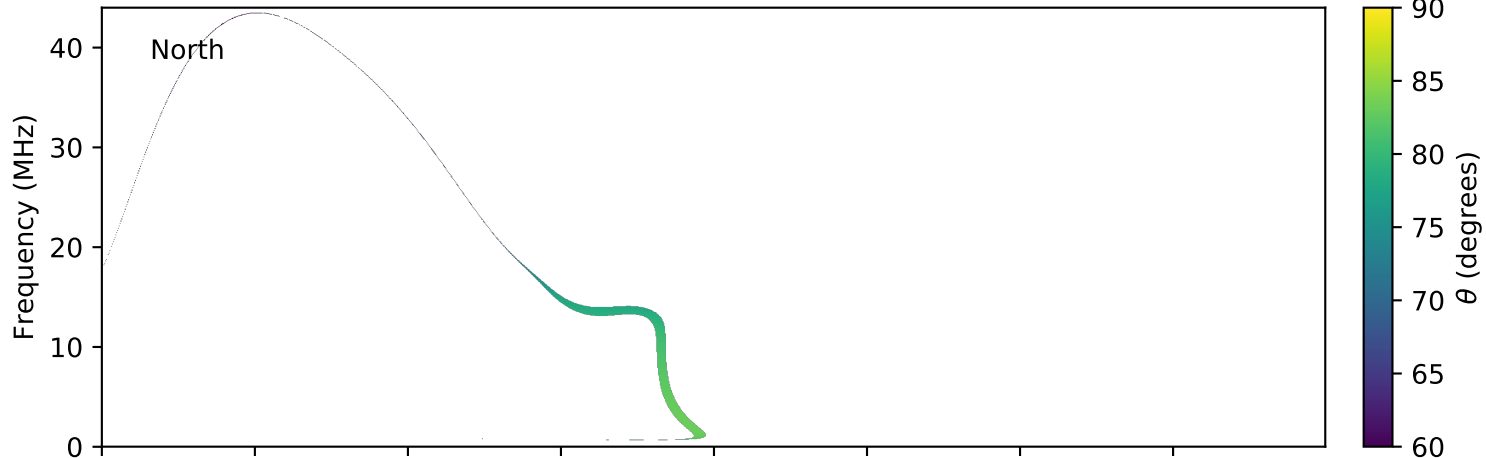
expres_earth_jupiter_io_jrm09_lossc-wid1deg_3kev_20160908_v01.cdf
