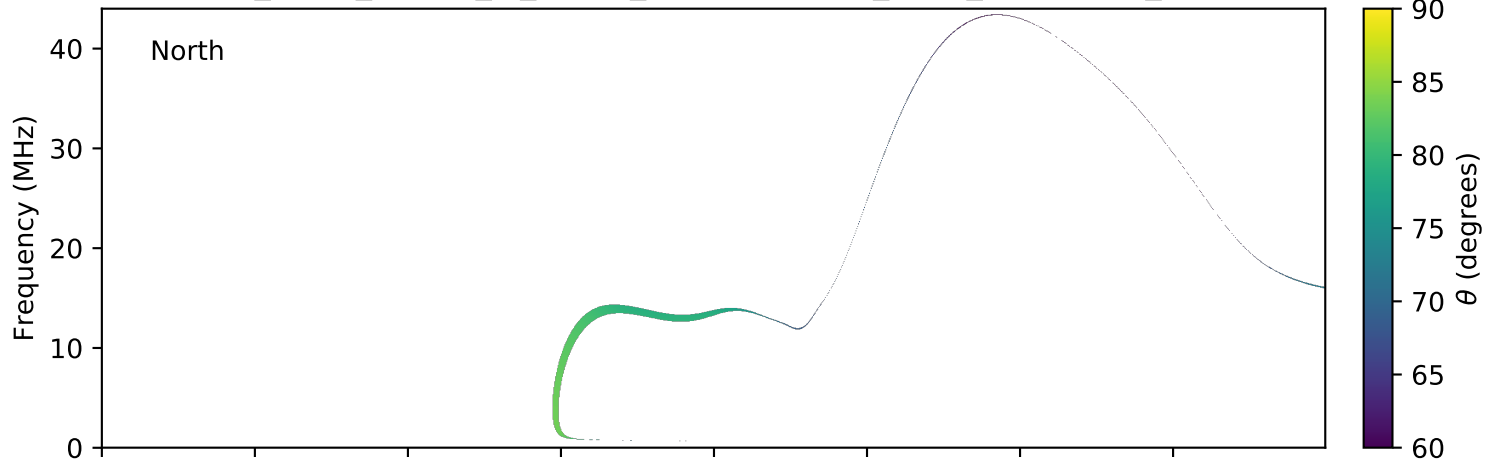
expres_earth_jupiter_io_jrm09_lossc-wid1deg_3kev_20160902_v01.cdf
