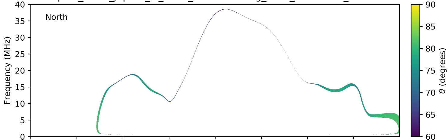
expres_earth_jupiter_io_isaac_lossc-wid1deg_5kev_20160927_v01.cdf
