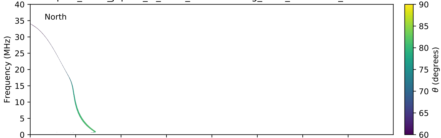
expres_earth_jupiter_io_isaac_lossc-wid1deg_5kev_20160926_v01.cdf
