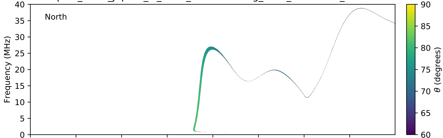
expres_earth_jupiter_io_isaac_lossc-wid1deg_5kev_20160925_v01.cdf
