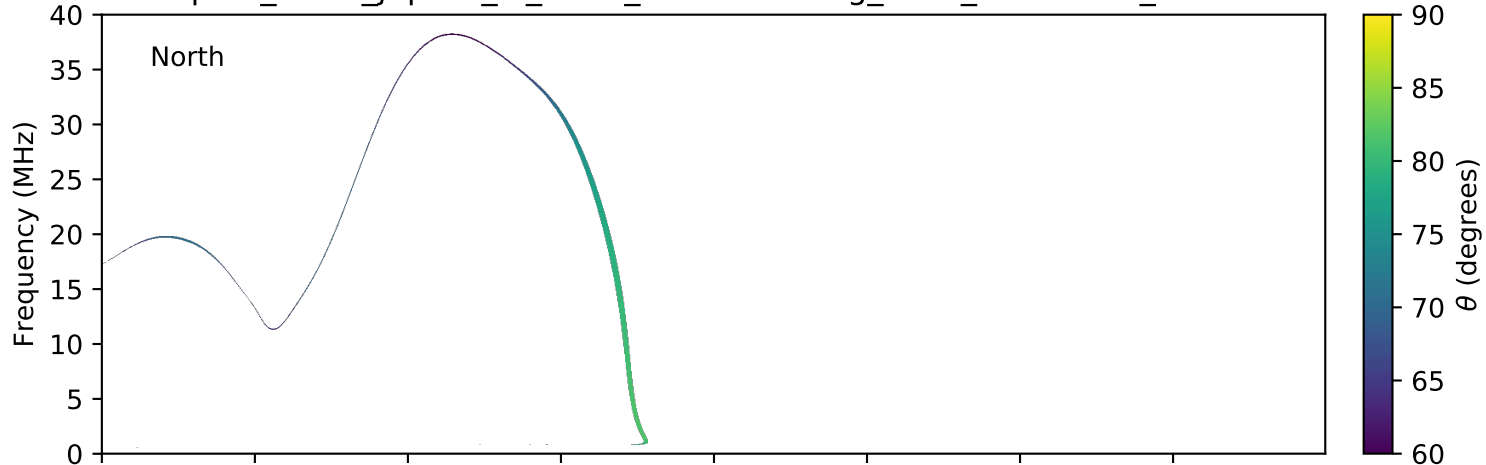
expres_earth_jupiter_io_isaac_lossc-wid1deg_5kev_20160924_v01.cdf
