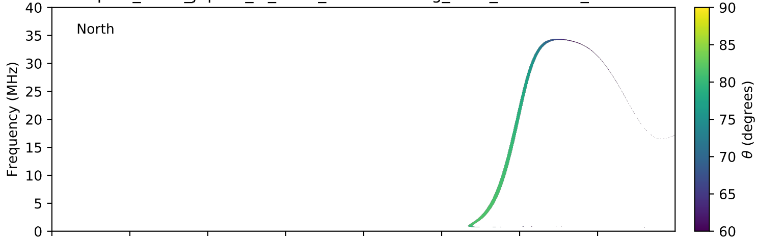
expres_earth_jupiter_io_isaac_lossc-wid1deg_5kev_20160923_v01.cdf
