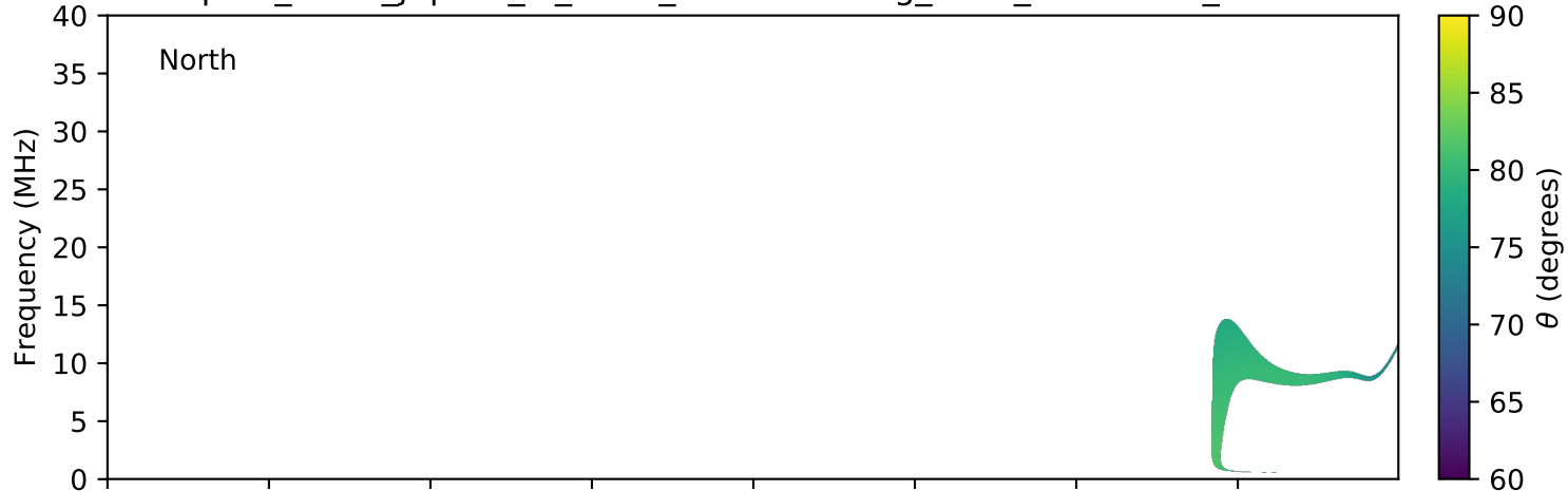
expres_earth_jupiter_io_isaac_lossc-wid1deg_5kev_20160921_v01.cdf
