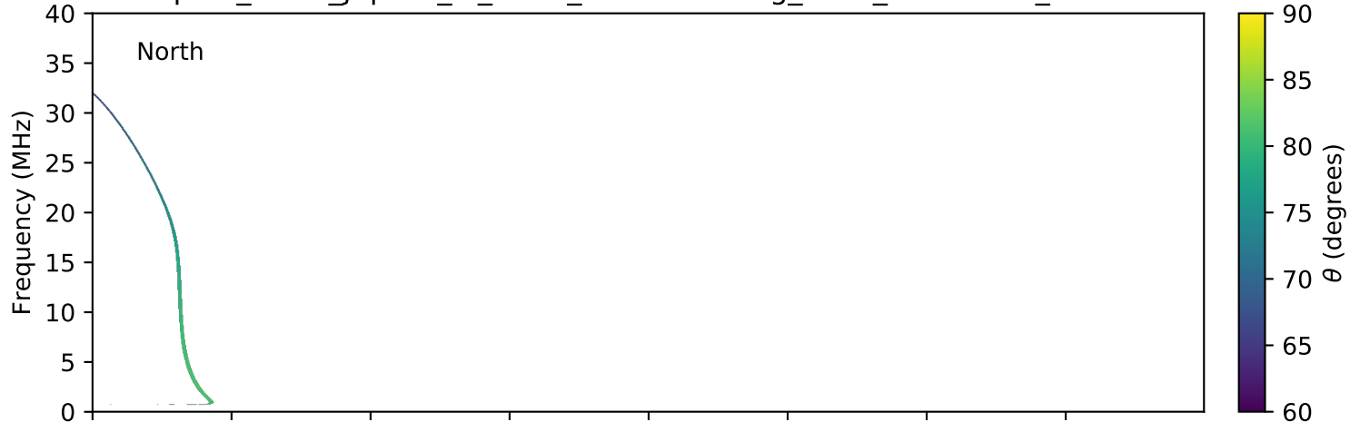
expres_earth_jupiter_io_isaac_lossc-wid1deg_5kev_20160919_v01.cdf
