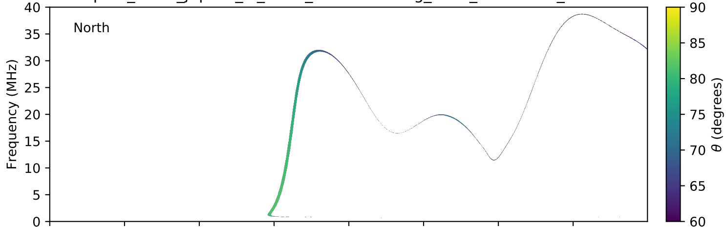
expres_earth_jupiter_io_isaac_lossc-wid1deg_5kev_20160918_v01.cdf
