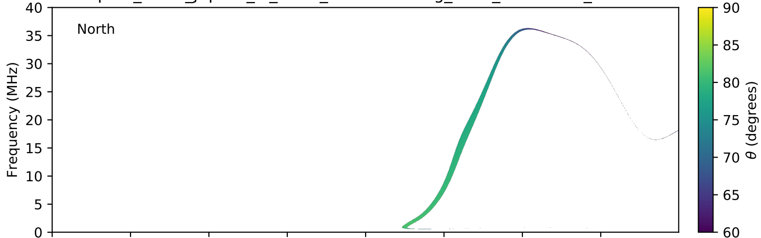
expres_earth_jupiter_io_isaac_lossc-wid1deg_5kev_20160916_v01.cdf
