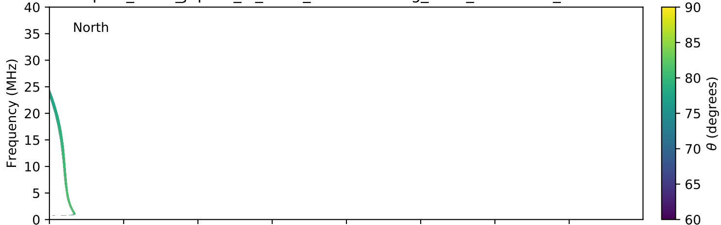
expres_earth_jupiter_io_isaac_lossc-wid1deg_5kev_20160912_v01.cdf
