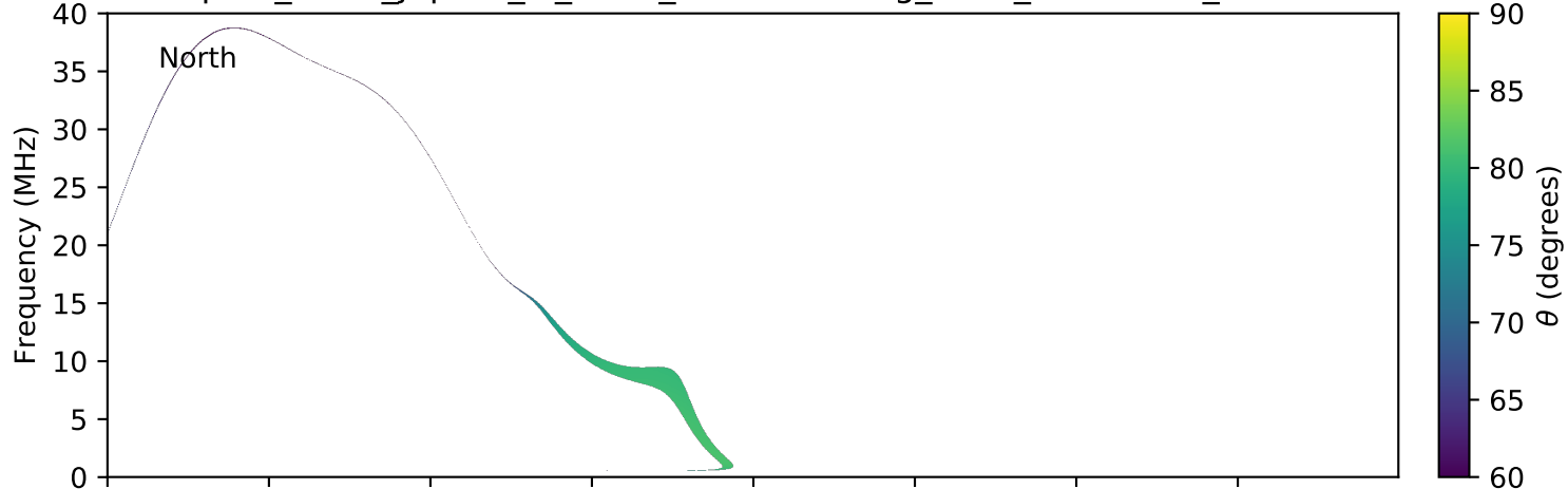
expres_earth_jupiter_io_isaac_lossc-wid1deg_5kev_20160908_v01.cdf
