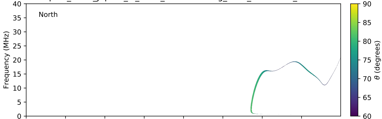
expres_earth_jupiter_io_isaac_lossc-wid1deg_5kev_20160907_v01.cdf
