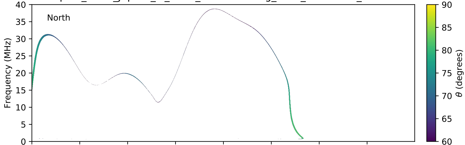
expres_earth_jupiter_io_isaac_lossc-wid1deg_5kev_20160906_v01.cdf
