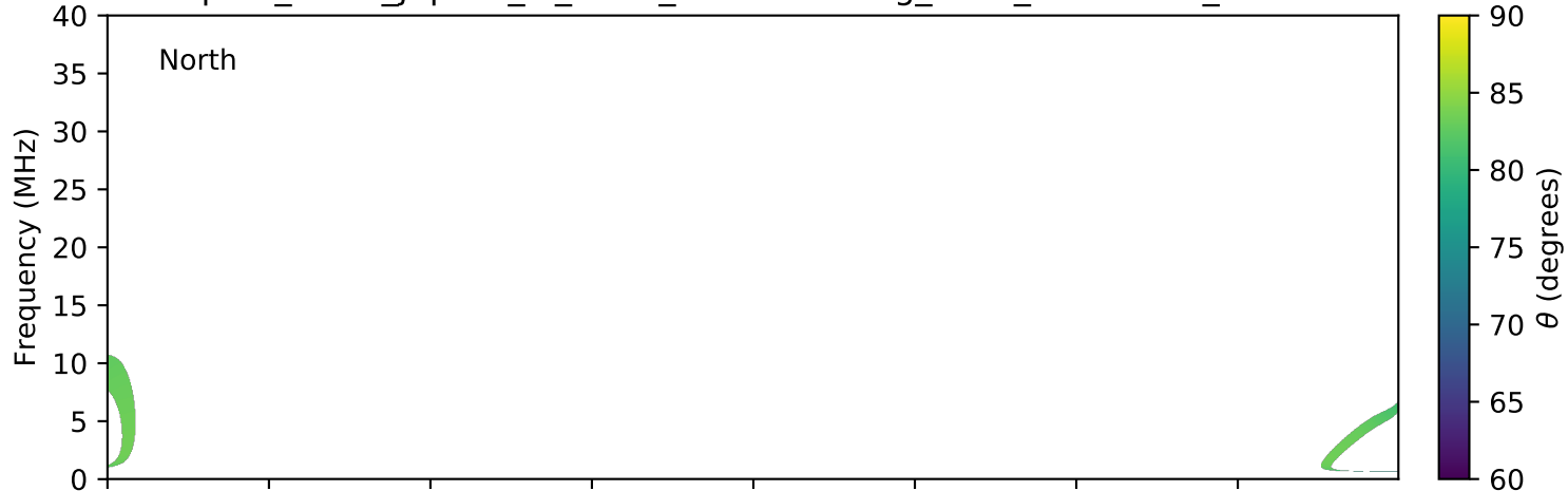
expres_earth_jupiter_io_isaac_lossc-wid1deg_3kev_20160928_v01.cdf
