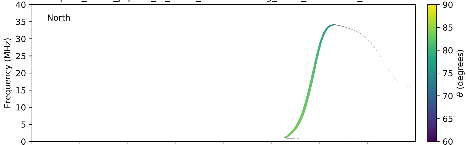
expres_earth_jupiter_io_isaac_lossc-wid1deg_3kev_20160923_v01.cdf
