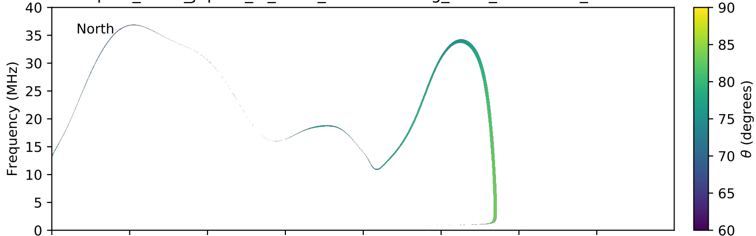
expres_earth_jupiter_io_isaac_lossc-wid1deg_3kev_20160922_v01.cdf
