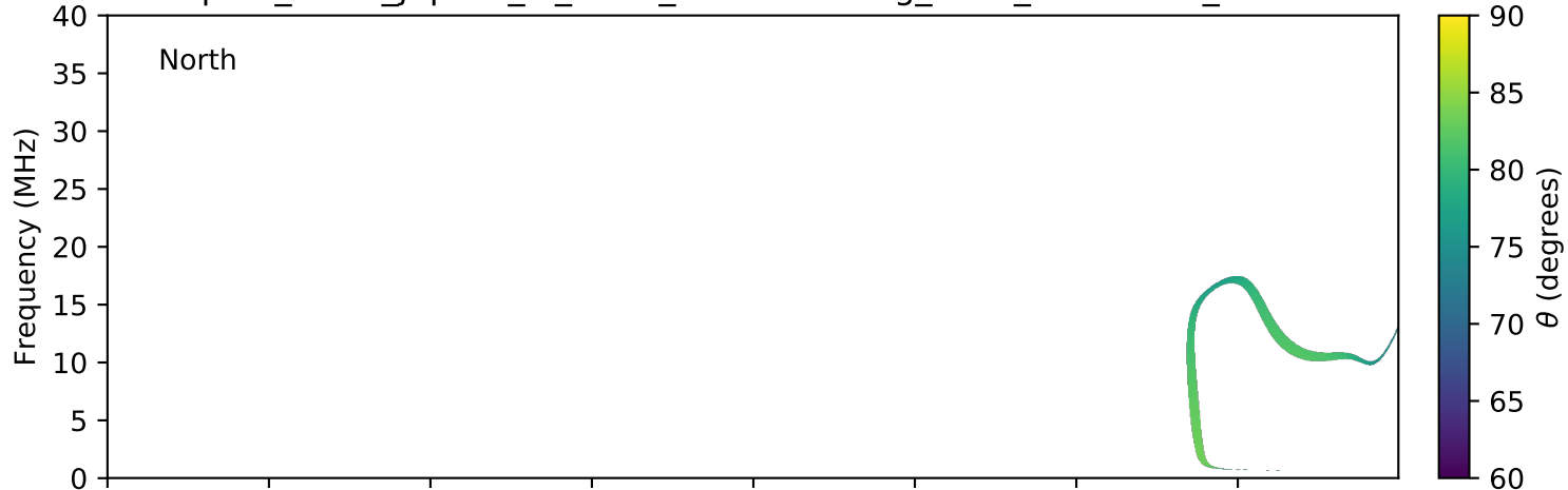
expres_earth_jupiter_io_isaac_lossc-wid1deg_3kev_20160921_v01.cdf
