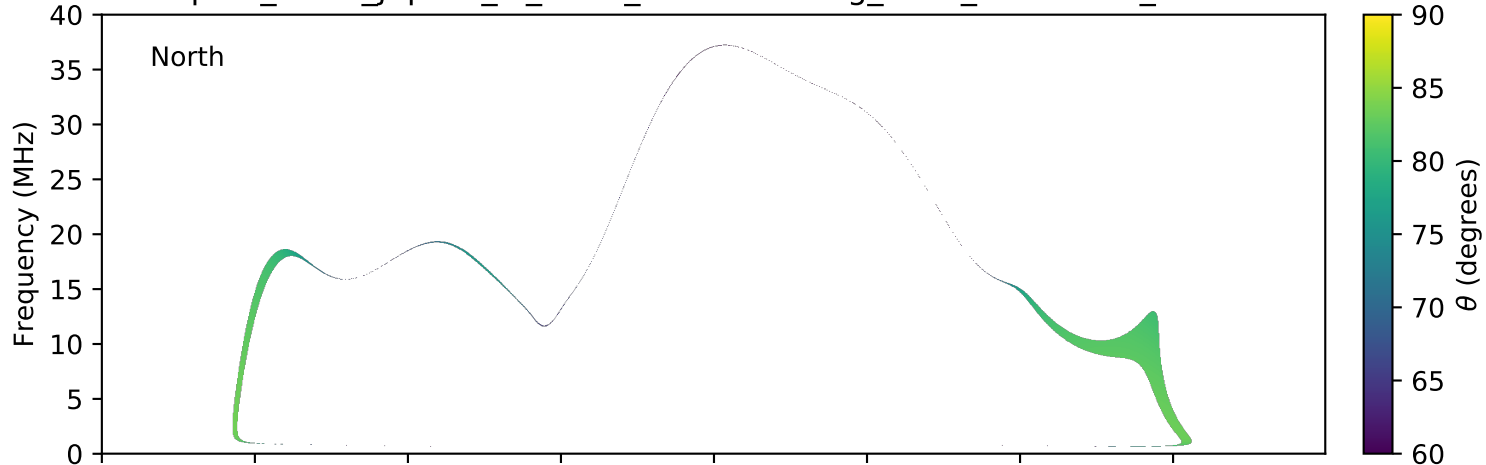
expres_earth_jupiter_io_isaac_lossc-wid1deg_3kev_20160920_v01.cdf
