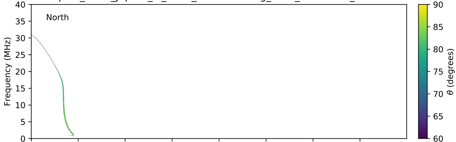
expres_earth_jupiter_io_isaac_lossc-wid1deg_3kev_20160919_v01.cdf
